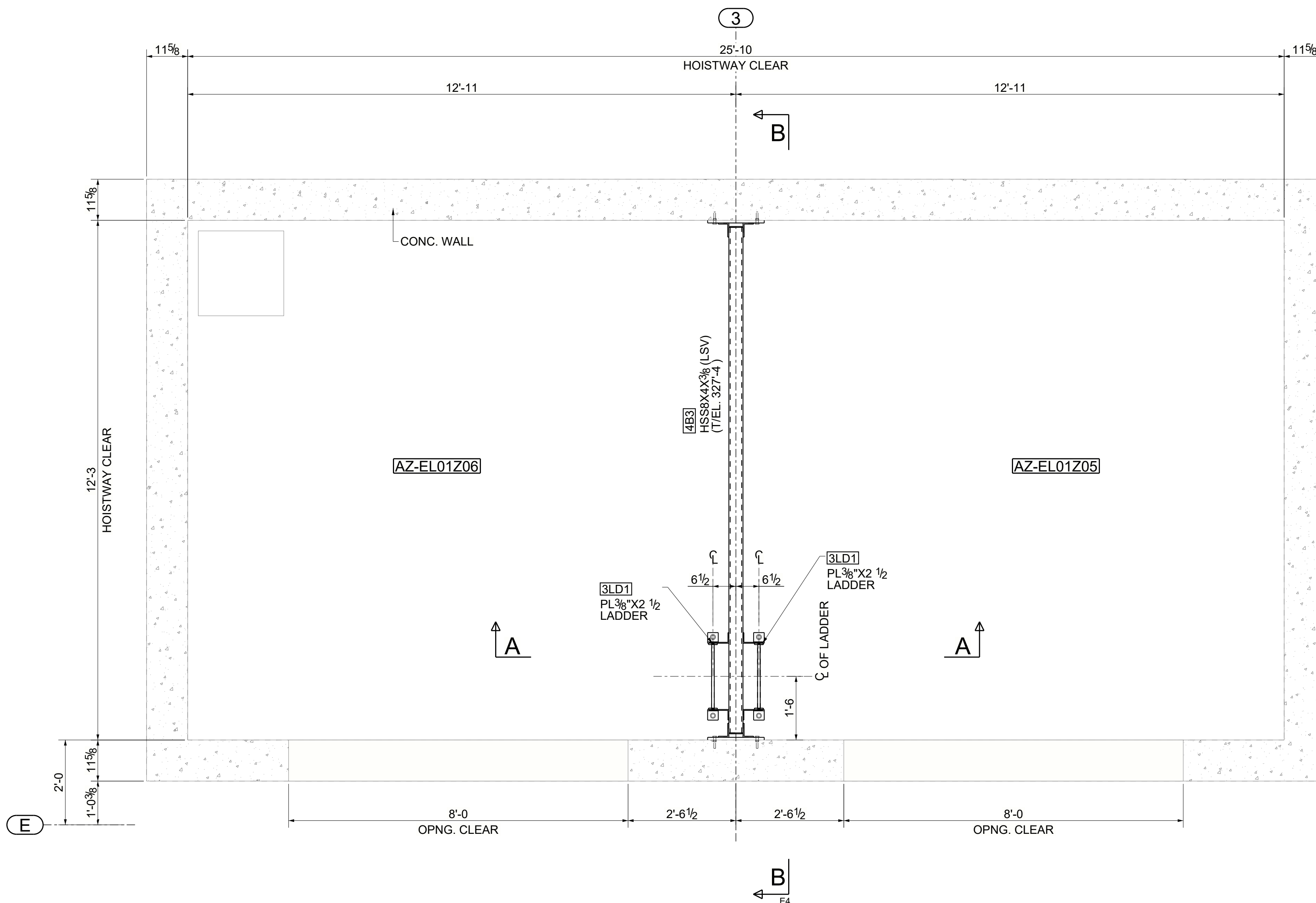
SERVICE ELEVATOR -PIT LADDER LOCATION PLAN (REFER : SERVICE ELEVATORS -ELEVATOR PIT PLAN-1/A644-A5300301 & A644-S3000004)
