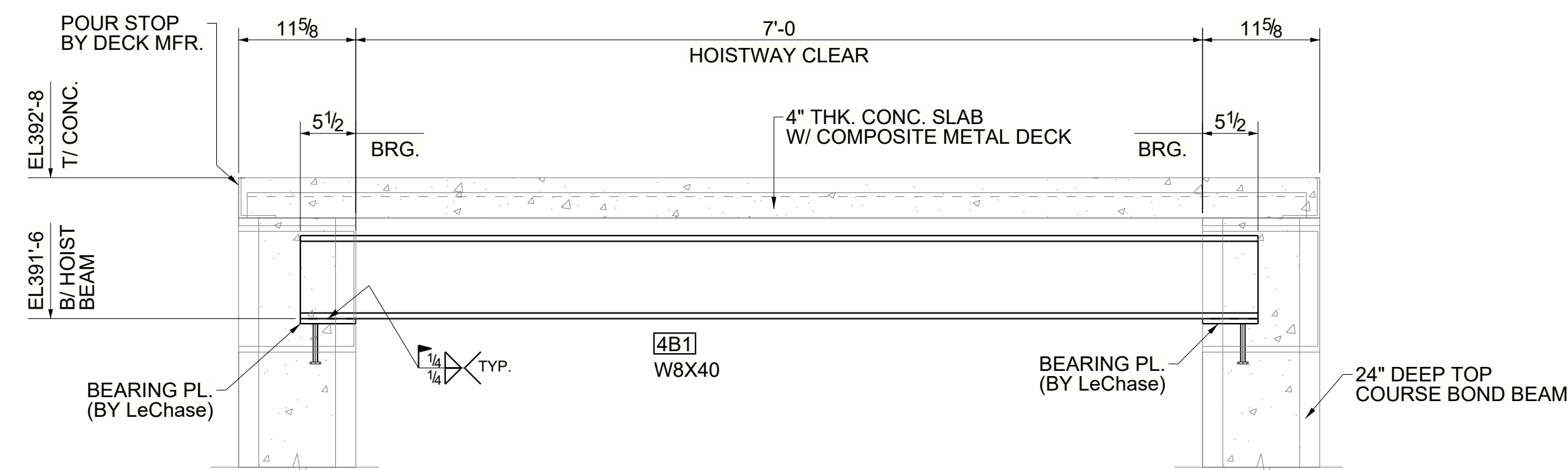
SECTION B - B (REFER : SECTION-1/ A644-S3000004)
