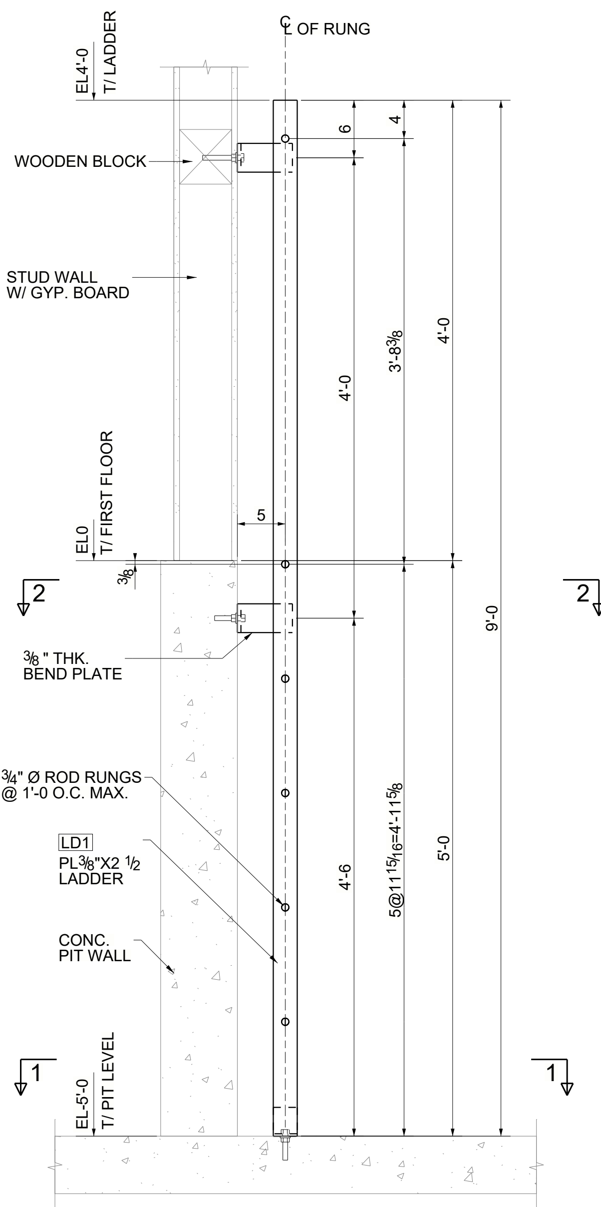
SECTION A - A
