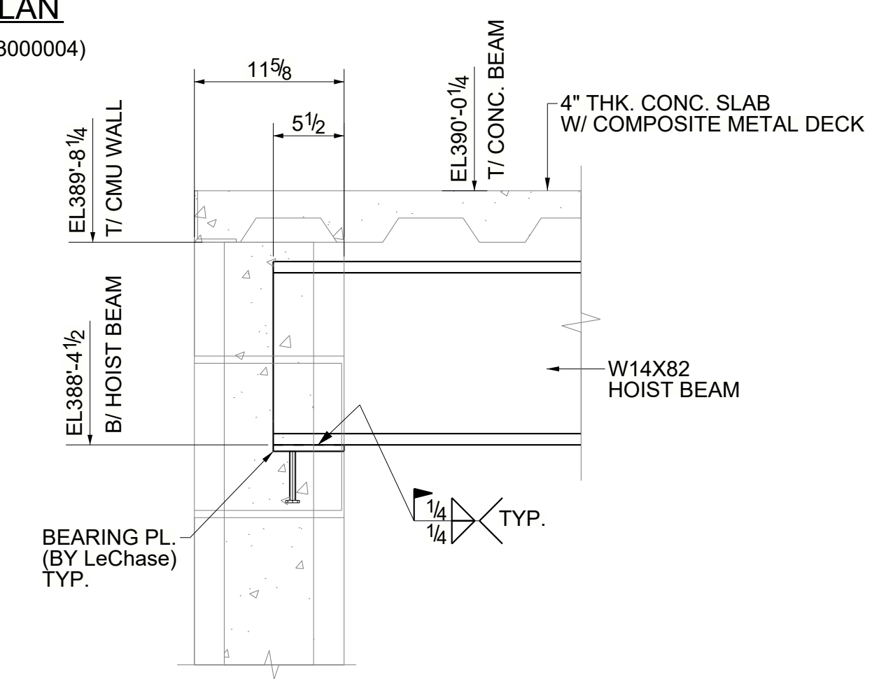
SECTION 1A - 1A (REFER : SECTION-3/ A644-S3000004)
