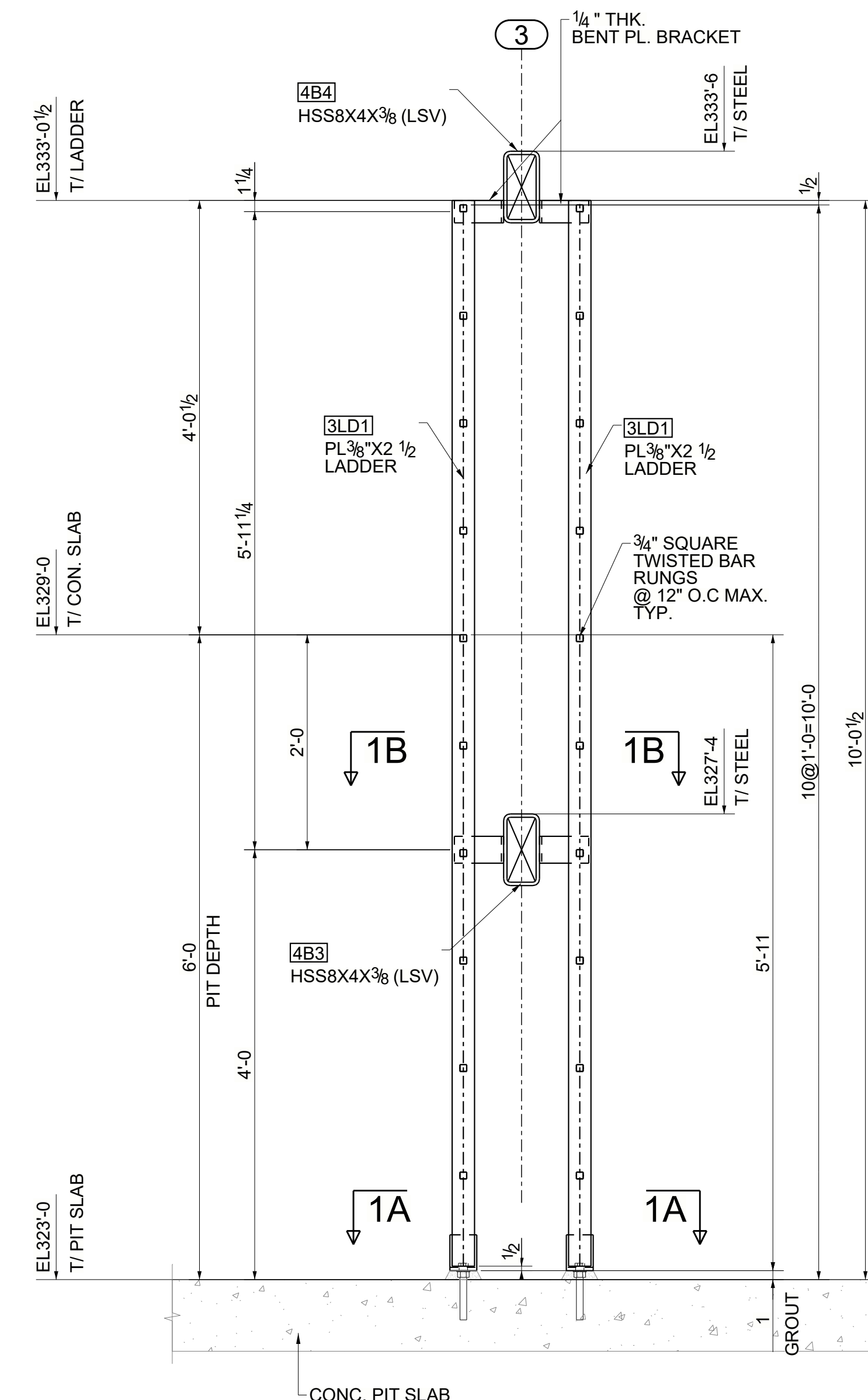
SECTION A - A (REFER : SECTION -6 /A644-A3000004)
