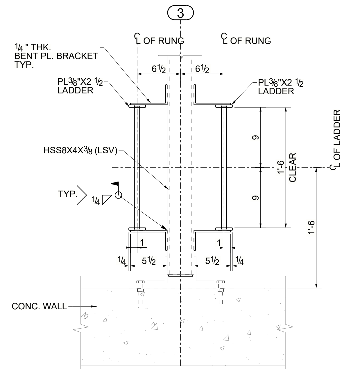
SECTION 1B - 1B
