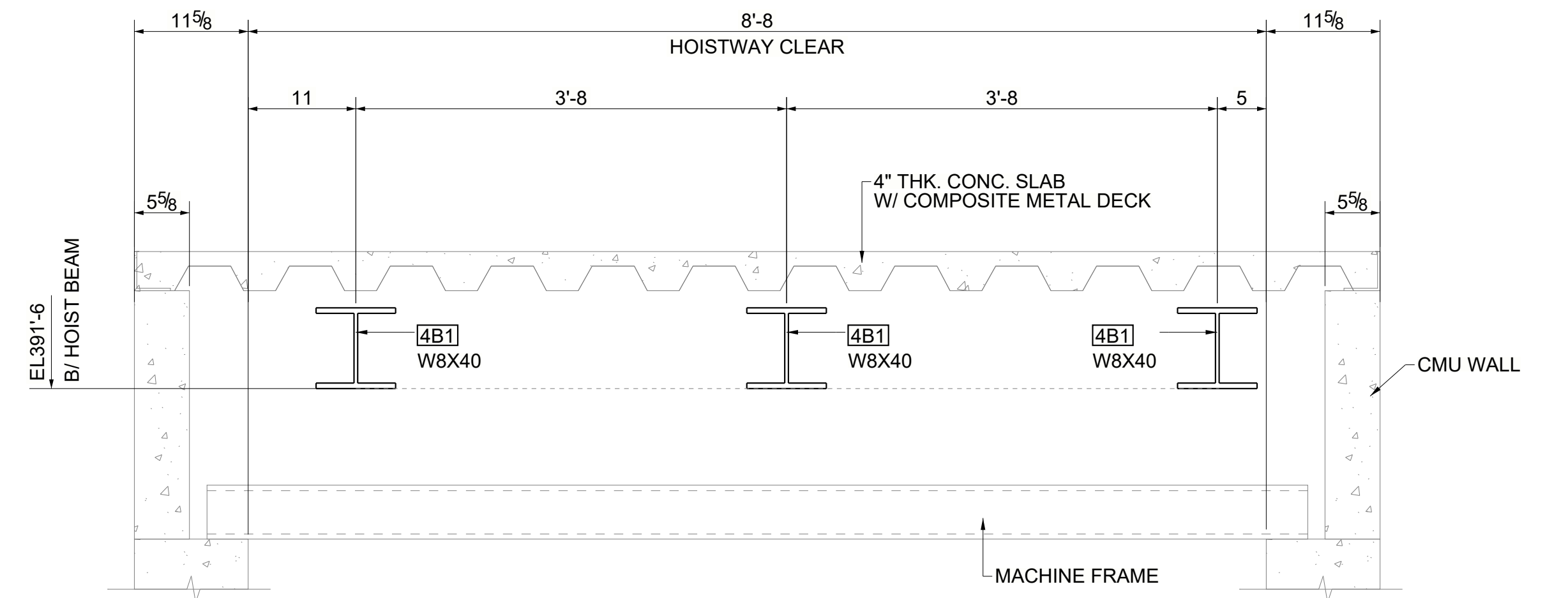
SECTION A - A (REFER : SECTION-2/ A644-S3000004)
