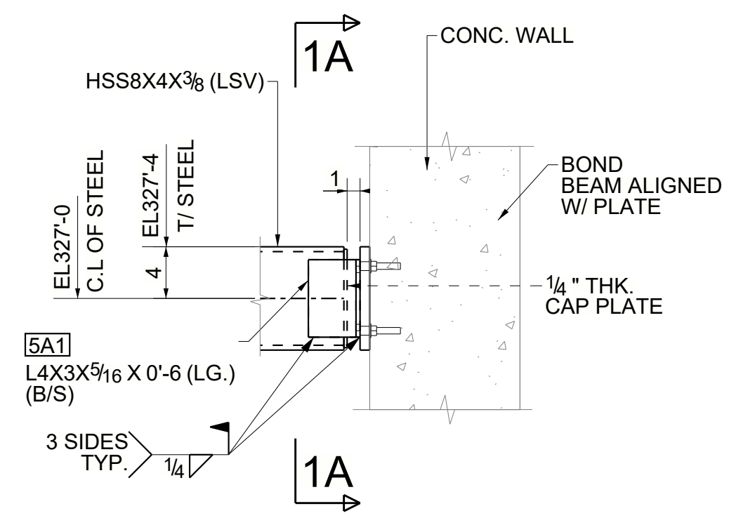
DETAIL 1 (REFER : SECTION-5/ A644-S3000004)
