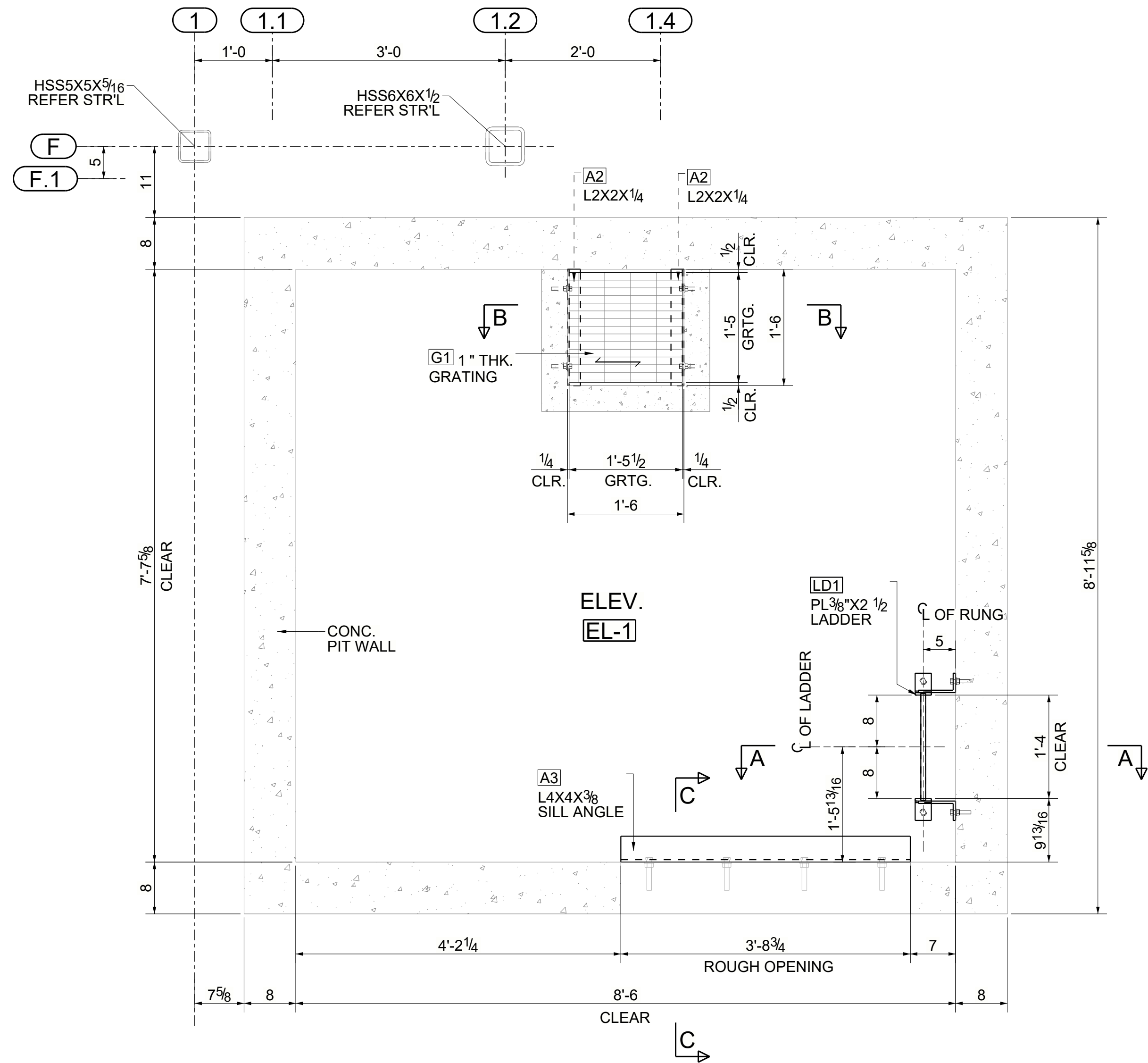
ELEVATOR PIT LADDER AND SUMP PIT GRATING LOCATION PLAN (REFER : ELEVATED ENLARGED PLAN - GROUND LEVEL/ 1/A710)
