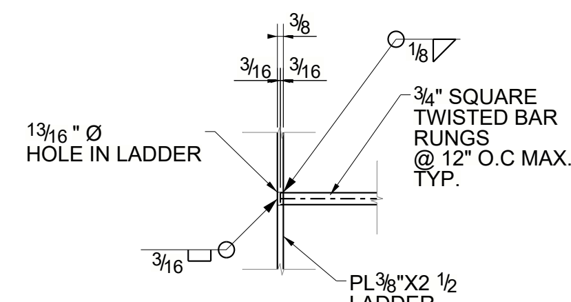
TYPICAL RUNG ATTACHMENT DETAIL (REFER : TYPICAL RUNG ATTACHMENT DETAIL /A644-S3000004)
