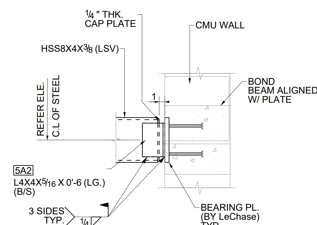
DETAIL 2 (REFER : SECTION-5/ A644-S3000004)
