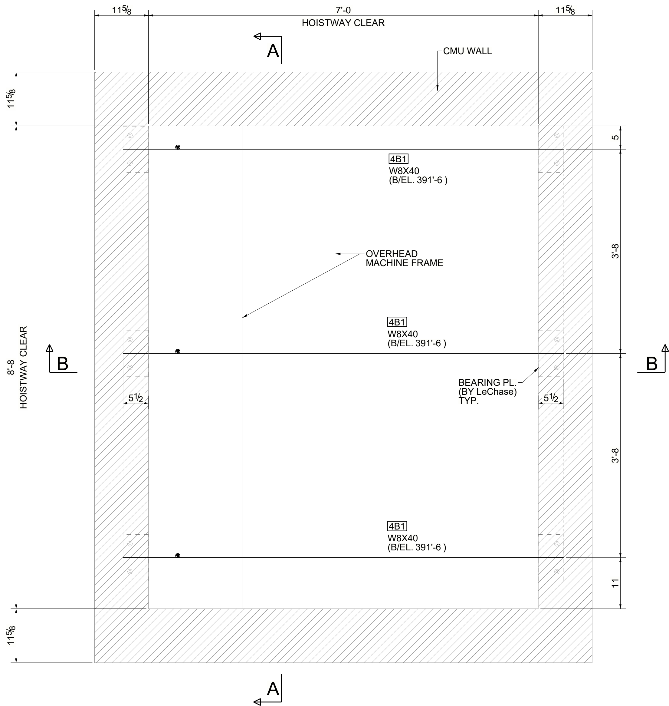
PERSONNEL ELEVATOR -HOISTWAY BEAM LOCATION PLAN (REFER : PERSONNEL ELEVATOR -HOISTWAY CAP PLAN-6/A644-A5300301 & A644-S3000004)
