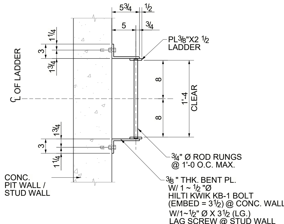
SECTION 2 - 2
