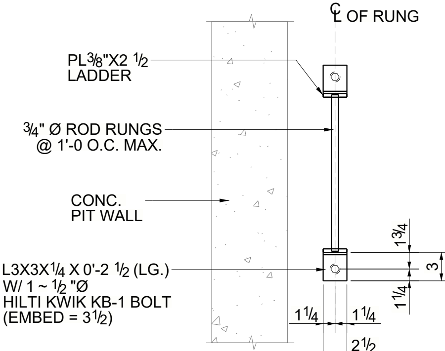
SECTION 1 - 1
