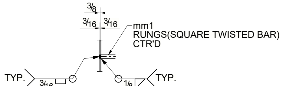
DETAIL 1
