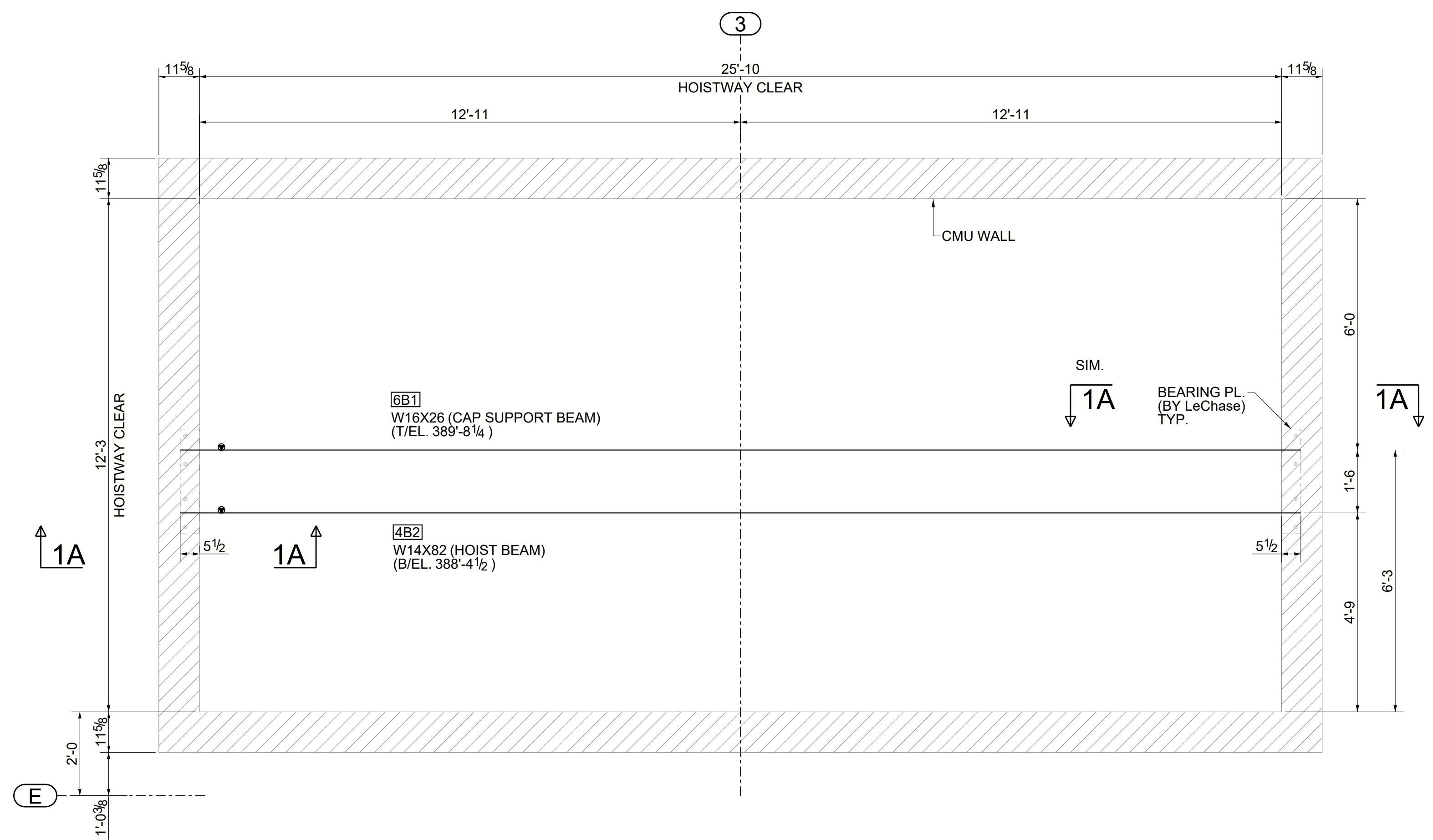
SERVICE ELEVATOR -HOISTWAY BEAM LOCATION PLAN (REFER : SERVICE ELEVATORS -HOISTWAY CAP PLAN - 3/A644-A5300301 & A644-S3000004)
