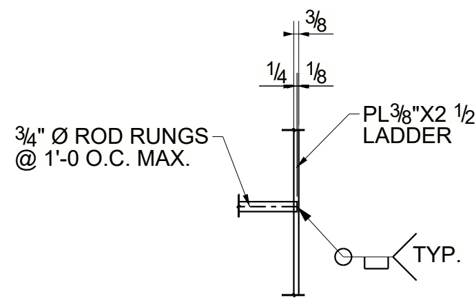
TYPICAL RUNG DETAIL
