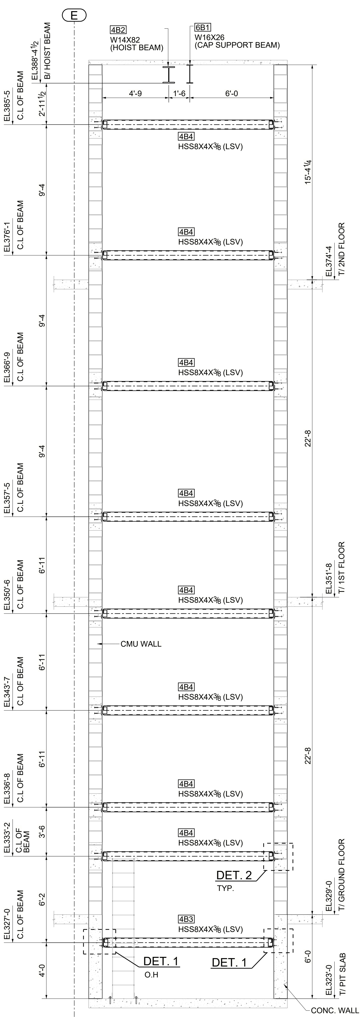
SECTION B - B E3 (REFER : SSECTION -SERVICE ELEVATORS N/S-7/A644-A5300301)
